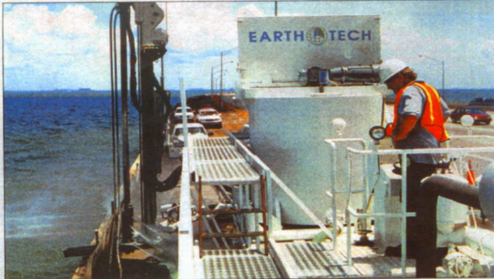
Earth Tech is constructing 3.6 miles of jet grouted wall along the Howard Frankland Bridge.
